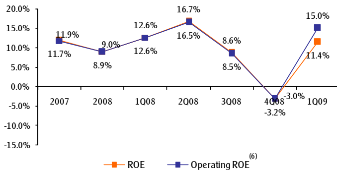
ROE Evolution
